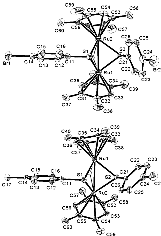
Figure 2. Molecular structures of [2c][BF 4 ] (top) and [2d][BF 4 ] (bottom); tetrafluoroborate anions and H atoms have been omitted for clarity; displacement ellipsoids are drawn at the 35 and 50% probability level, respectively; selected bond lengths (Å) and angles (°) are listed in Table 1
