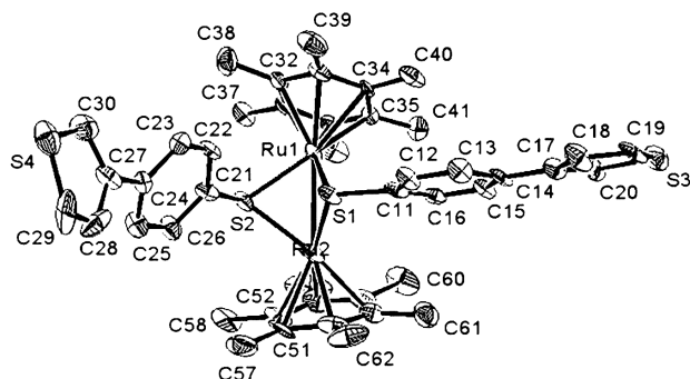
Figure 3. Molecular structure of [3][BF_4] ; the tetrafluoroborate anion, solvent molecule, and H atoms have been omitted for clarity; displacement ellipsoids are drawn at the 25% probability level; selected bond lengths (Å) and angles ( ^\circ ) are listed in Table 1
